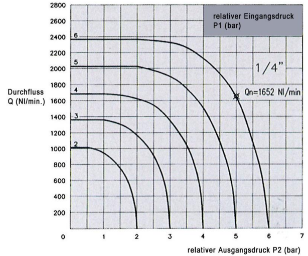
Type No. 377.02
