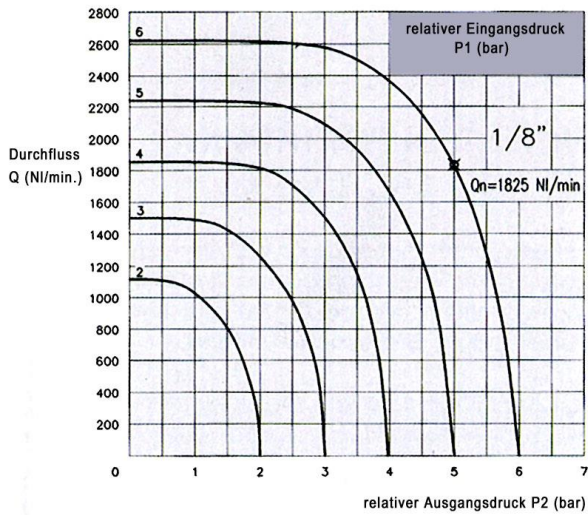
Type No. 377.01
