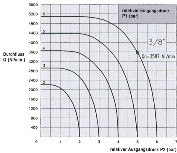
Type No. 377.03
